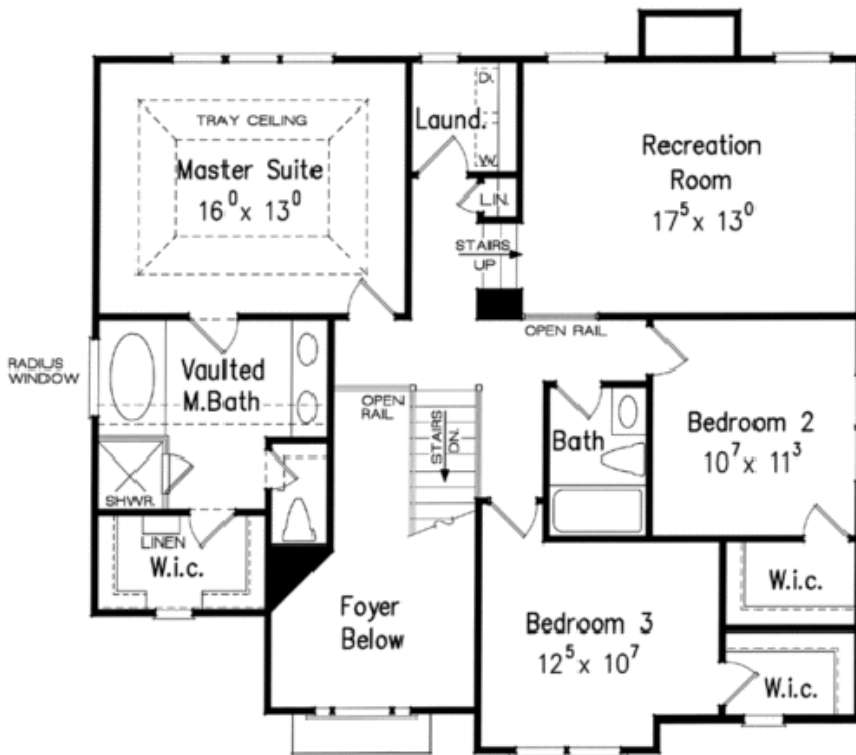
SECOND FLOOR
