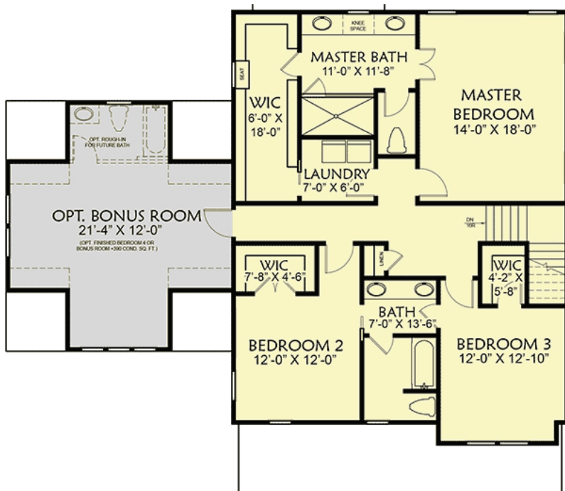
SECOND FLOOR
